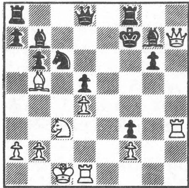
460 After 22 Rh3
